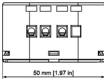
Fig. 8: Dimensions
