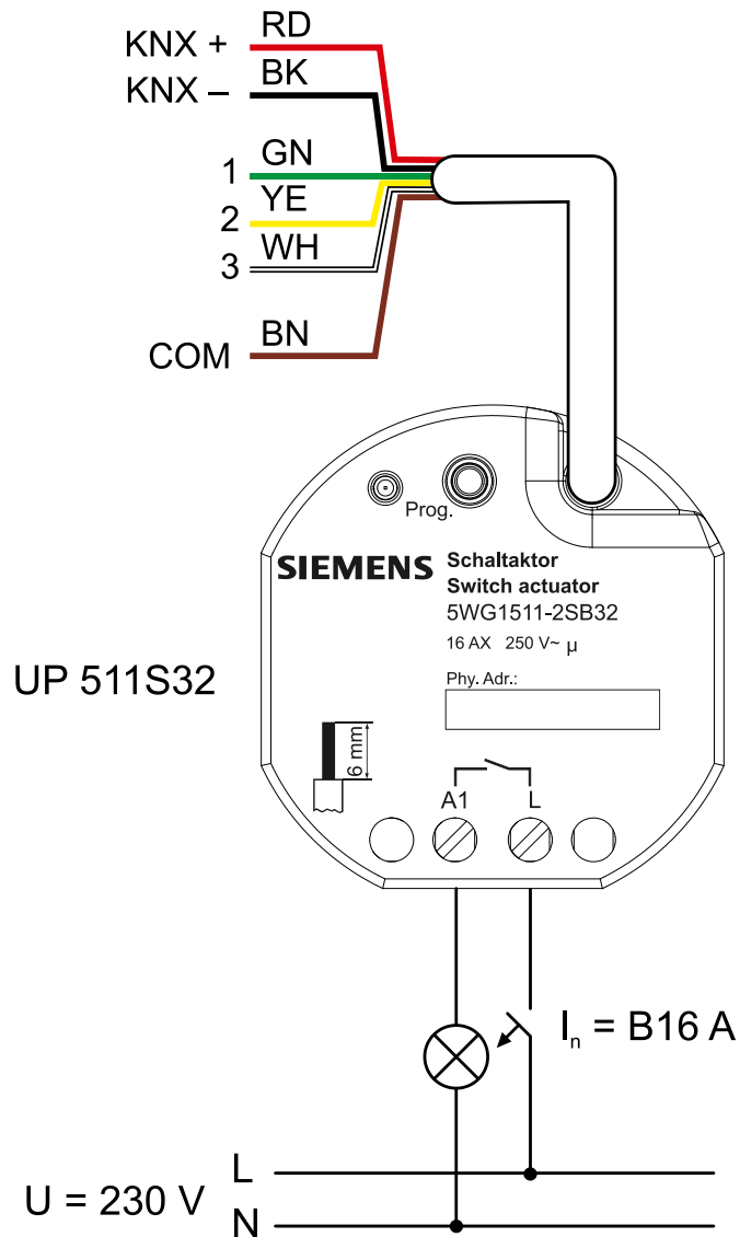
Fig. 7: Connection example for switching output
