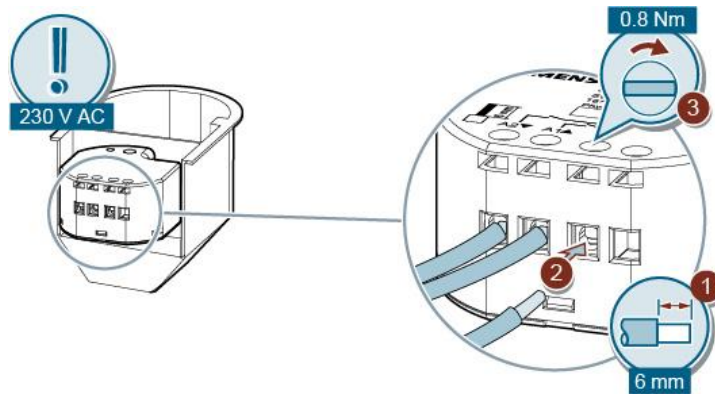
Fig. 3: Connecting loads to the switching contact
