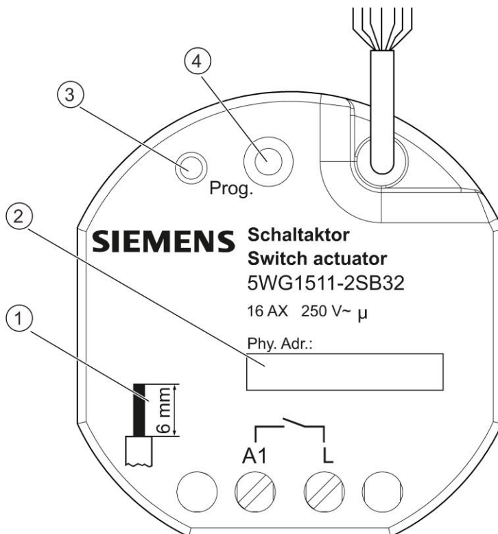
Fig. 2: Connections, operating and display elements
