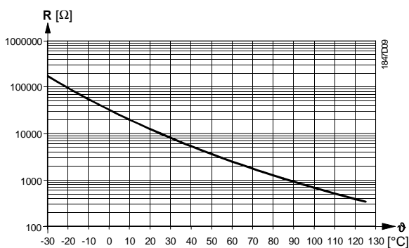
NTC 10k
